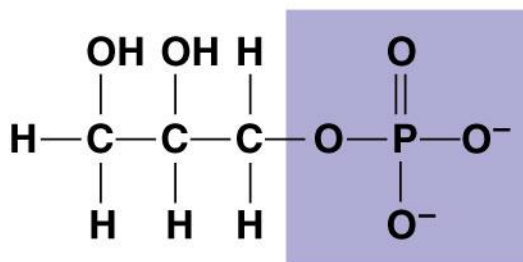
Glycerol phosphate
