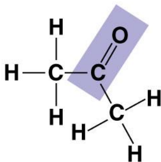
Acetone
