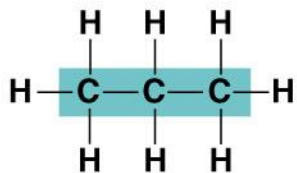
Propane
