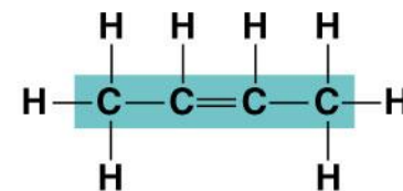
2-Butene
