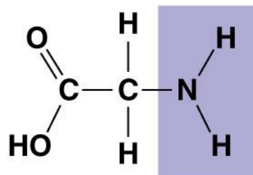
Glycine
